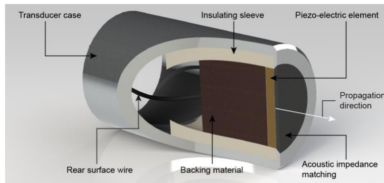
Figure 9 Components of a single-element transducer.
