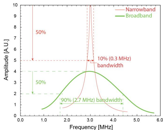
Figure 10 Tradeoff between higher-power output and wide bandwidth.
