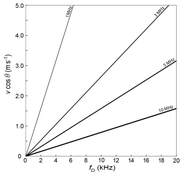
Figure 6 Lateral velocity as a function of Doppler shift at four different transmitting frequencies.
